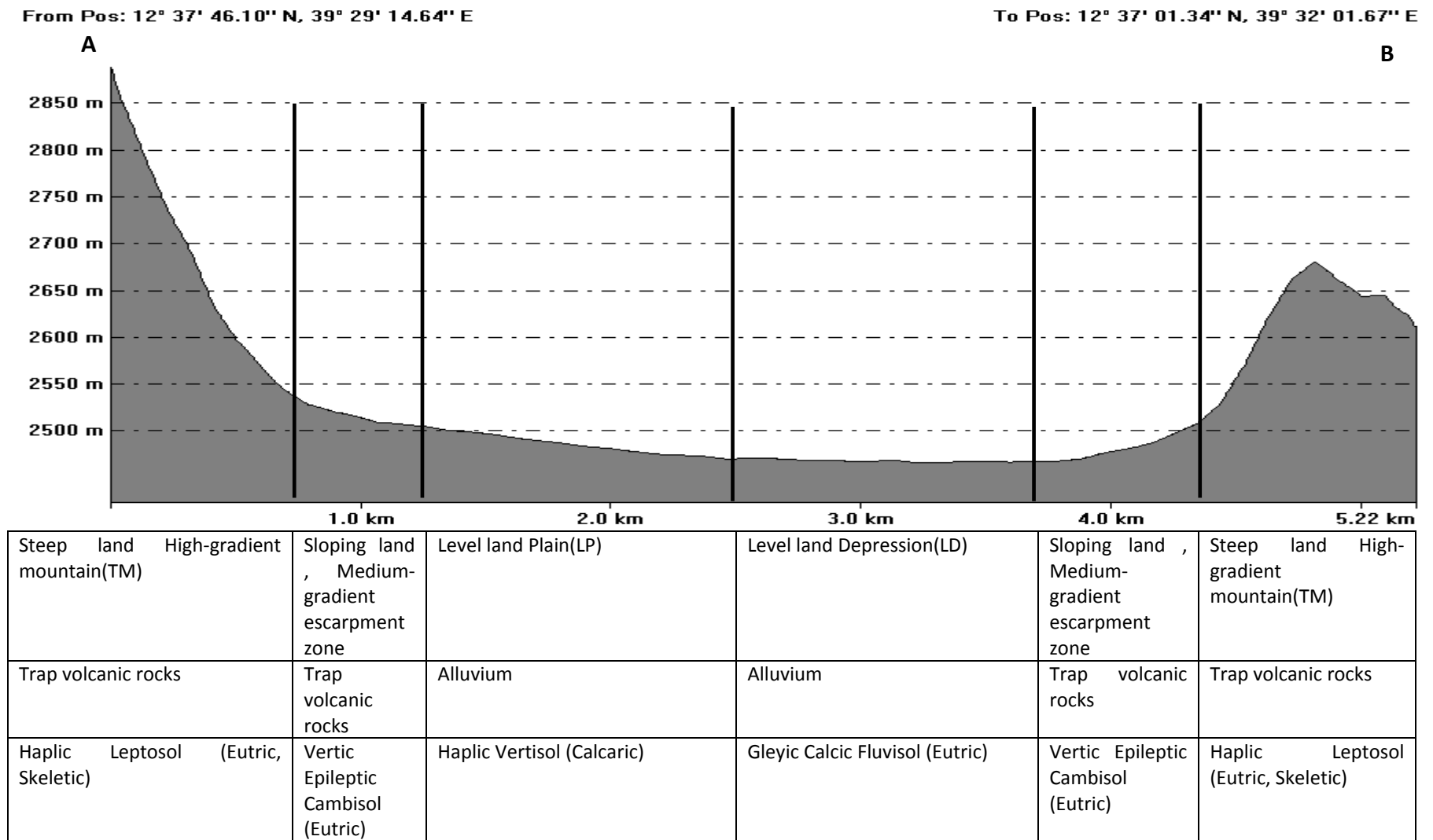
Figure 16 A: Cross profile AB dissected plateau at Menkere Kebele of Oflla woreda
