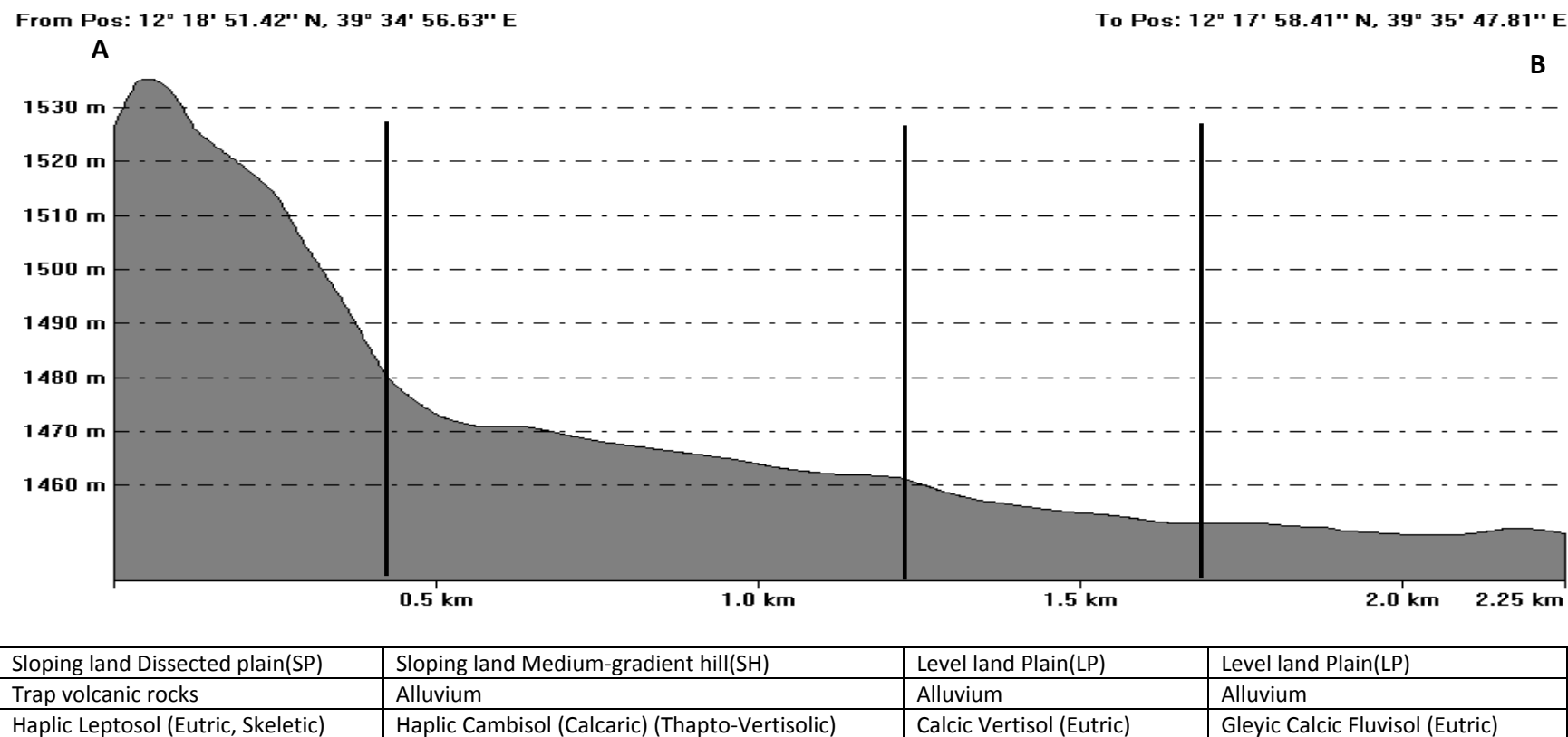
Figure 18A: Cross profile AB Graben valley at Tumuga Kebele of Raya Alamata woreda
