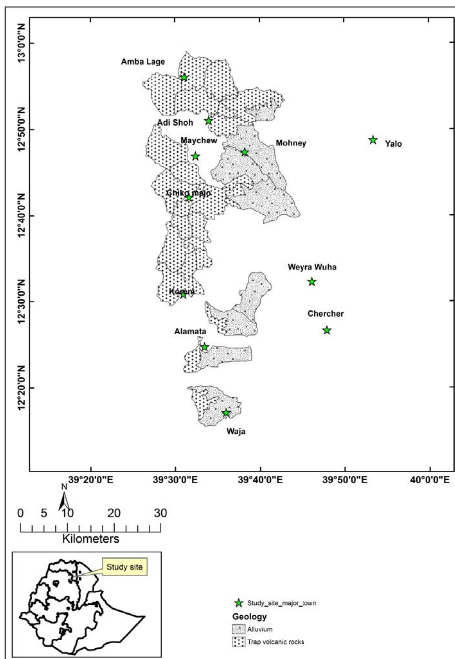
Figure 8: Geology map of the 5 CASCAPE intervention woredas Alaje, Enda Mokeni, Oflla, Raya Alamata and Raya Azebo in the regional cluster of Tigray, including 20 Kebeles.
